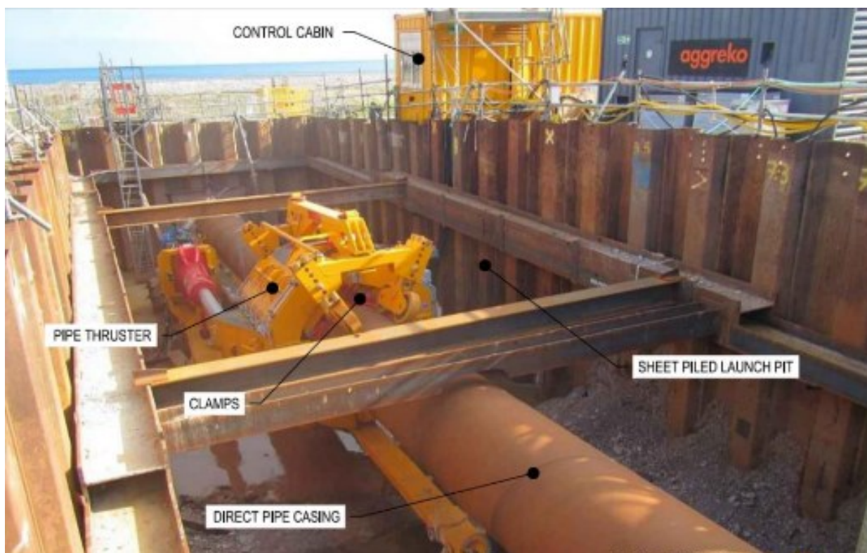
Figure 4.2526: Direct Pipe Installation
