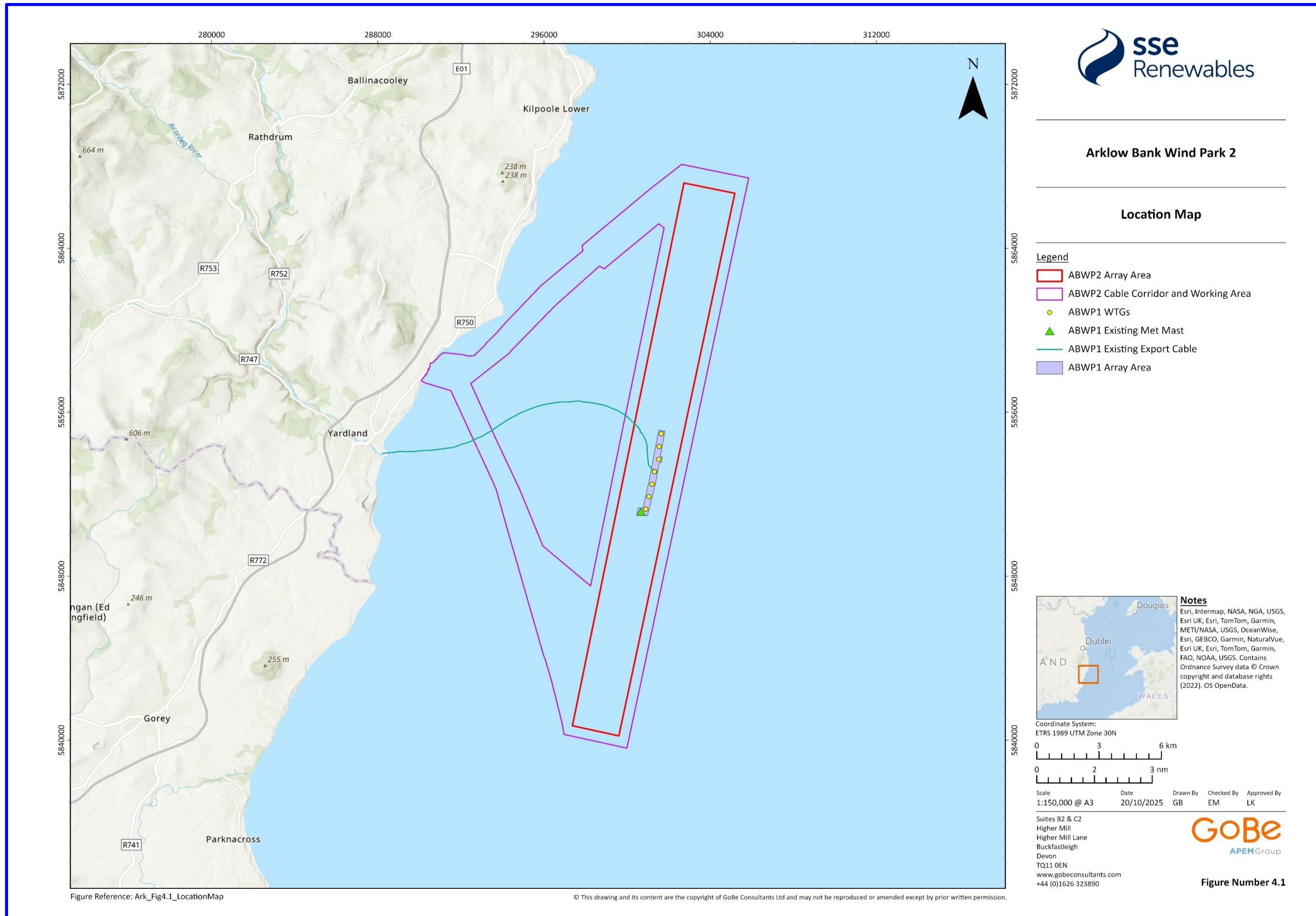
Figure 4.1: Arklow Bank Wind Park 2 Location Map
