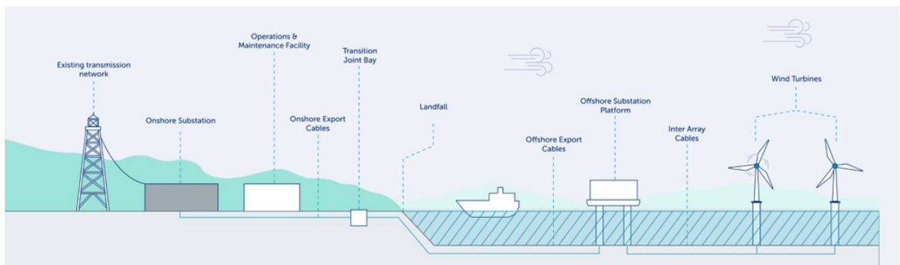
Figure 4.2: Main components of an offshore windfarm (OWF)
