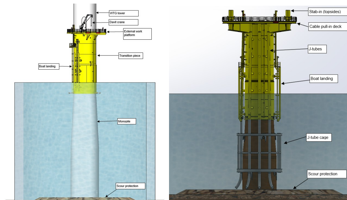
Figure 4.910: Typical monopile foundation general arrangement (left WTG, right OSP)
