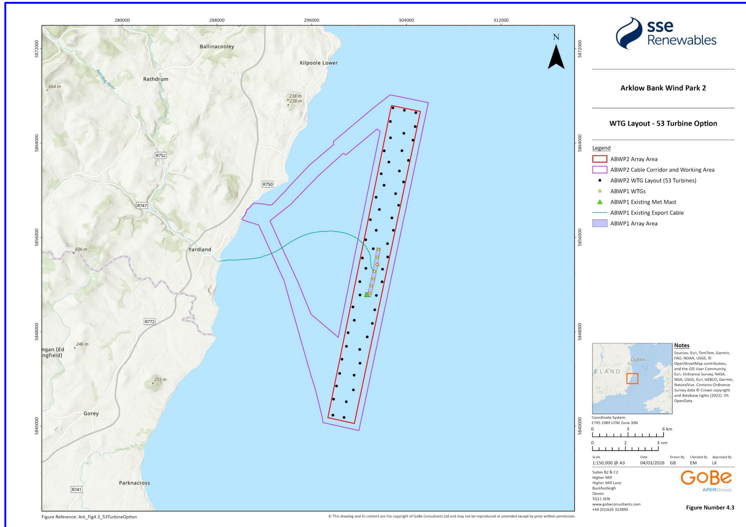
Figure 4.3: Proposed Development Project Design Option 1 (53 WTGs)
