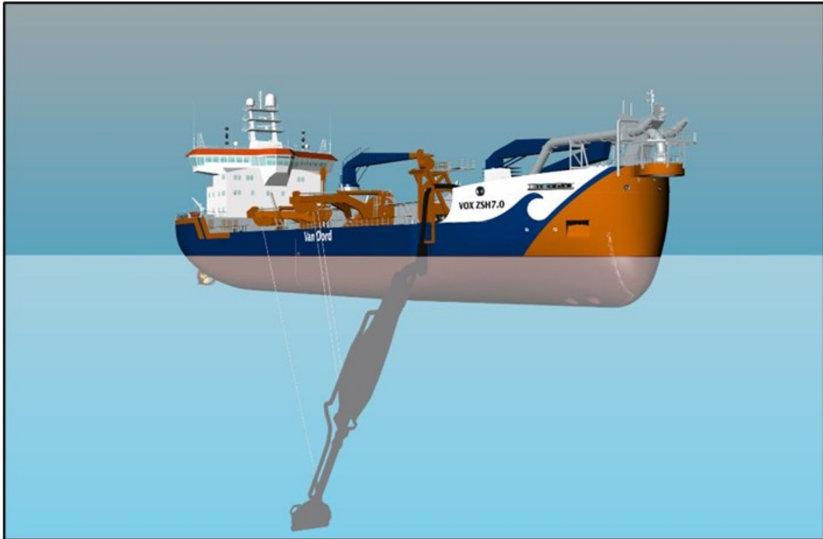
Figure 4.2021: Example of a seabed lowering/features clearance dredging vessel (Photo courtesy of Van Oord)
