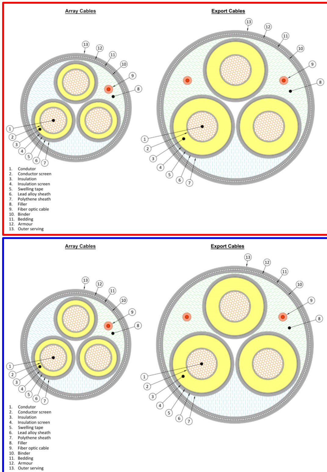
Figure 4.1112: Example of submarine cable cross section
