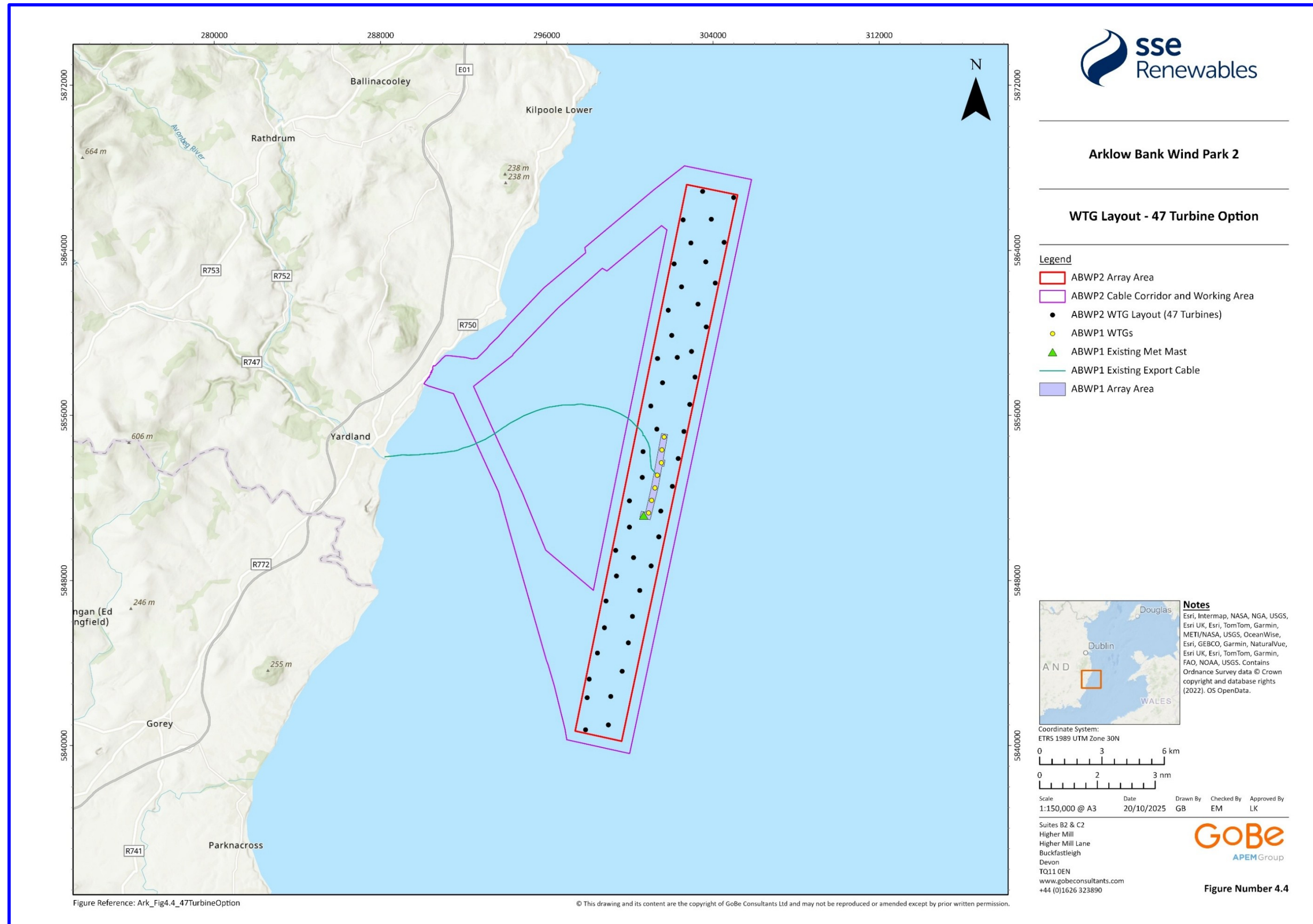
Figure 4.4: Proposed Development Project Design Option 2 (47 WTGs)
