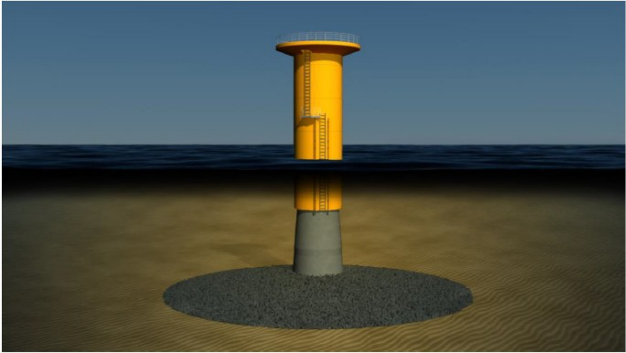
Figure 4.1011: Image showing Scour protection (Rock) installed around monopile (Image courtesy of Dogger Bank Windfarm)
